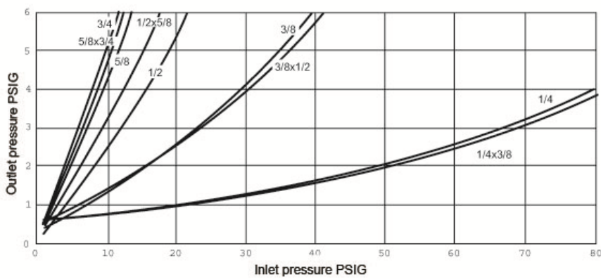
Relief Curves
