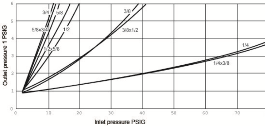
Relief Curves
