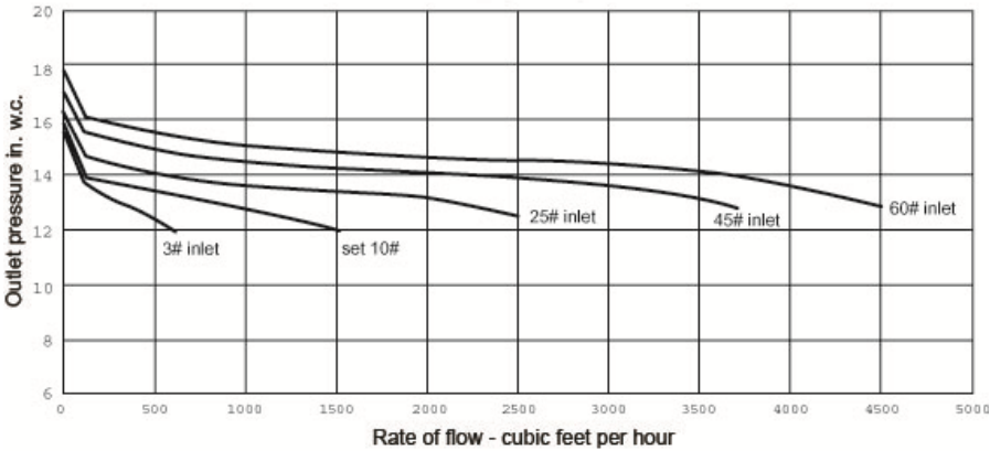
Performance Curves
