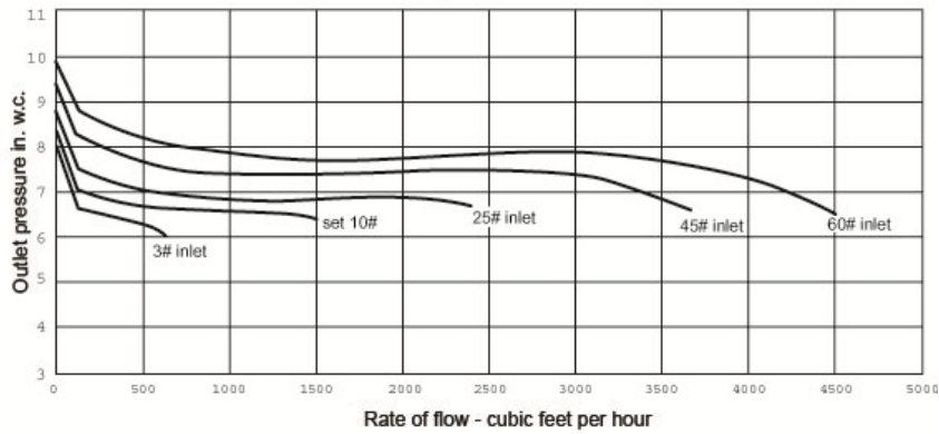
Relief Curves
